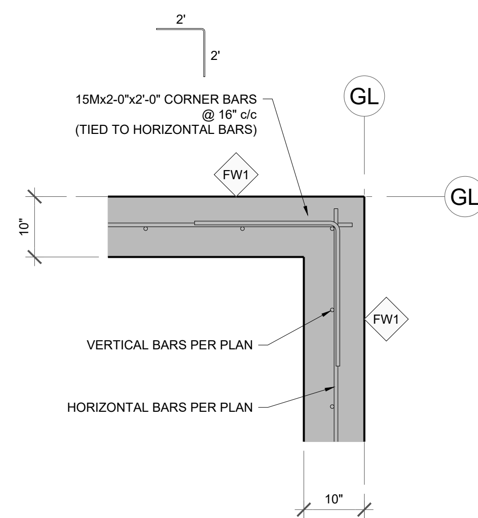
5 TYPICAL CORNER DETAIL U.N.O. S1.1 SCALE: 3/4"=1'-0"
