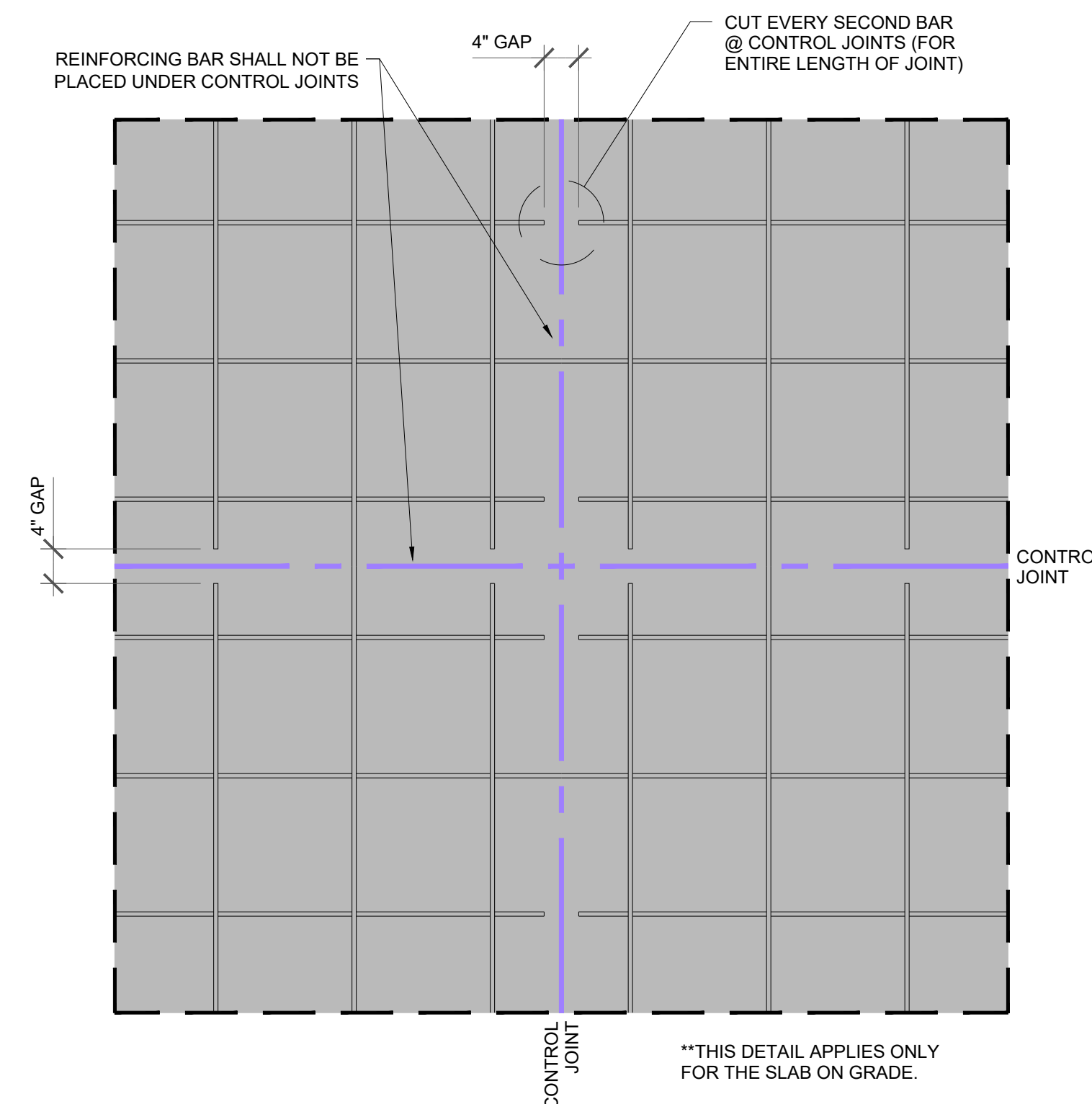
6 TYPICAL SLAB ON GRADE CONTROL JOINT DETAIL S1.1 SCALE: 3/4"=1'-0"
