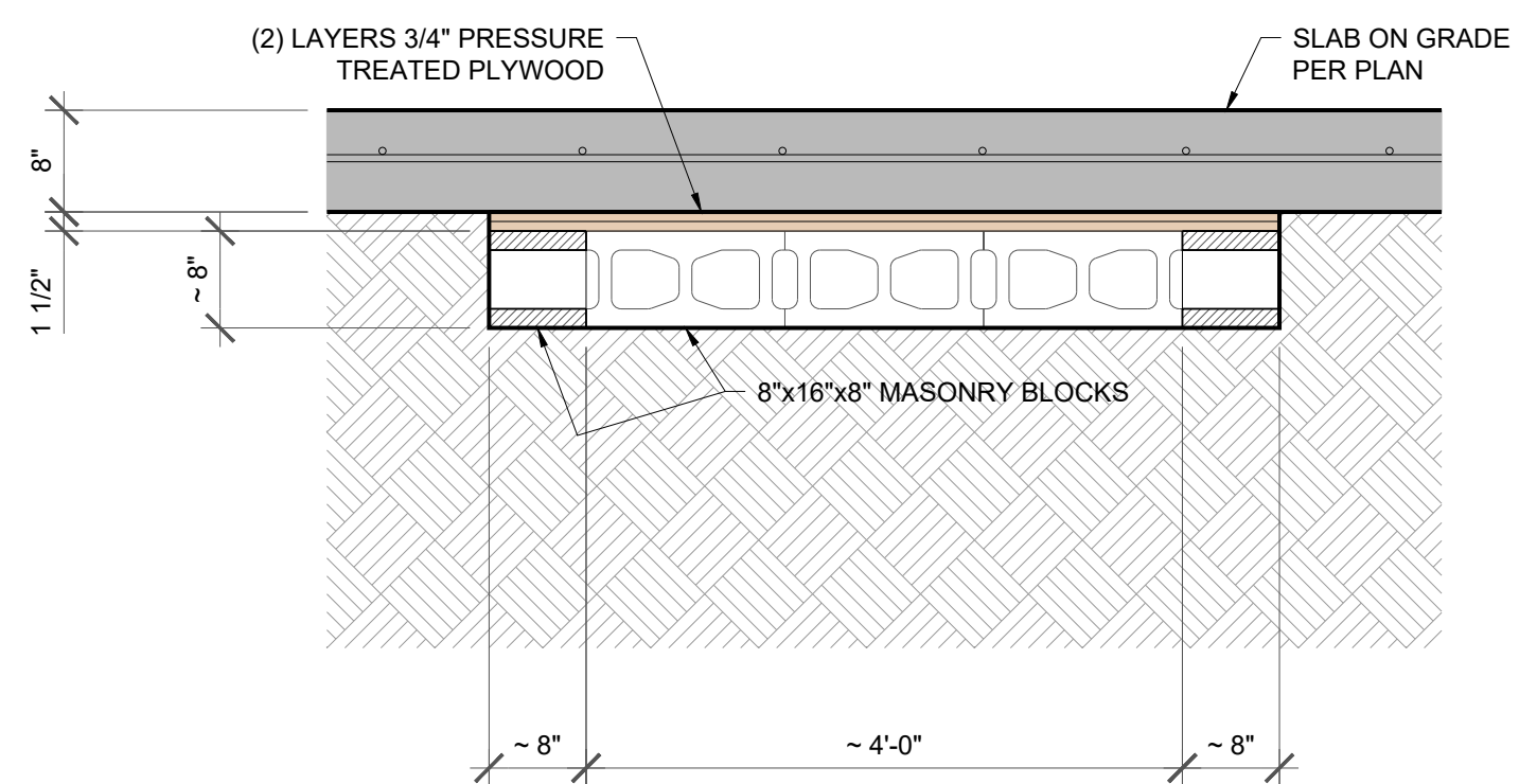
1 RADON PIT DETAIL S1.1 SCALE: 3/4"=1'-0"
